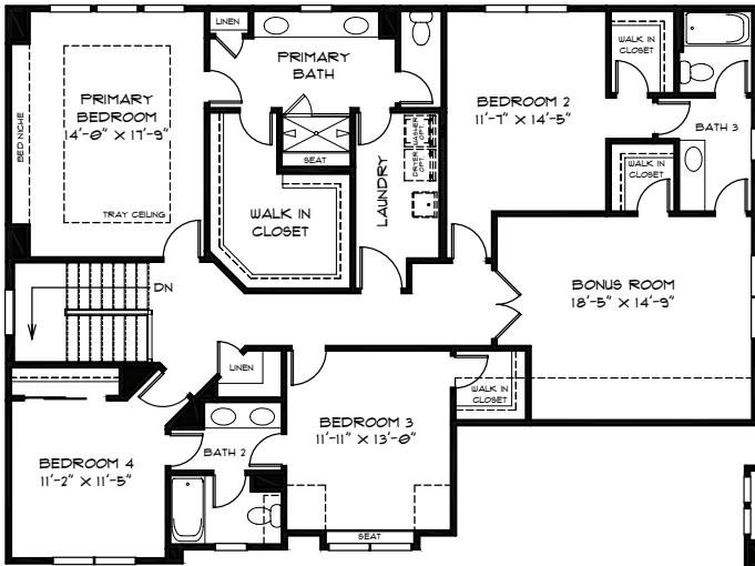
SECOND FLOOR
